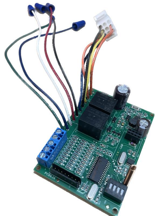
Figure 16. Control Board or "CB"
