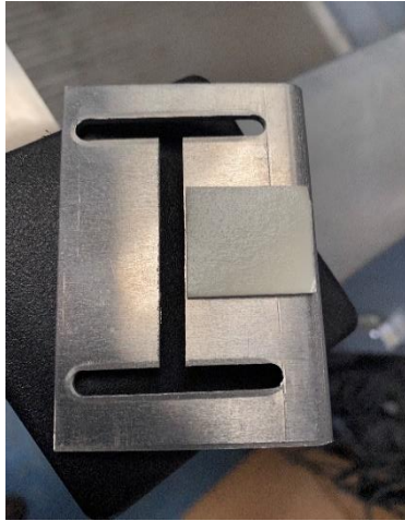
Figure 12. Two-sided tape on the bracket
