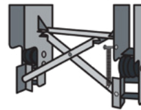
Automatic braking system stops lift instantly
